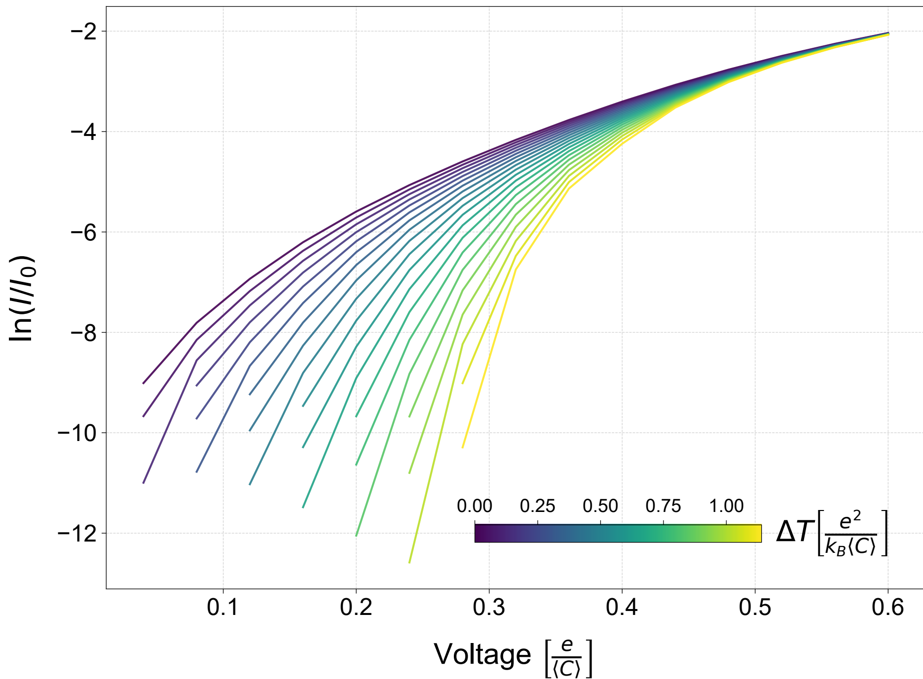
Semi-Log I-V for Fixed Island Temperature T = 1.2E_c
